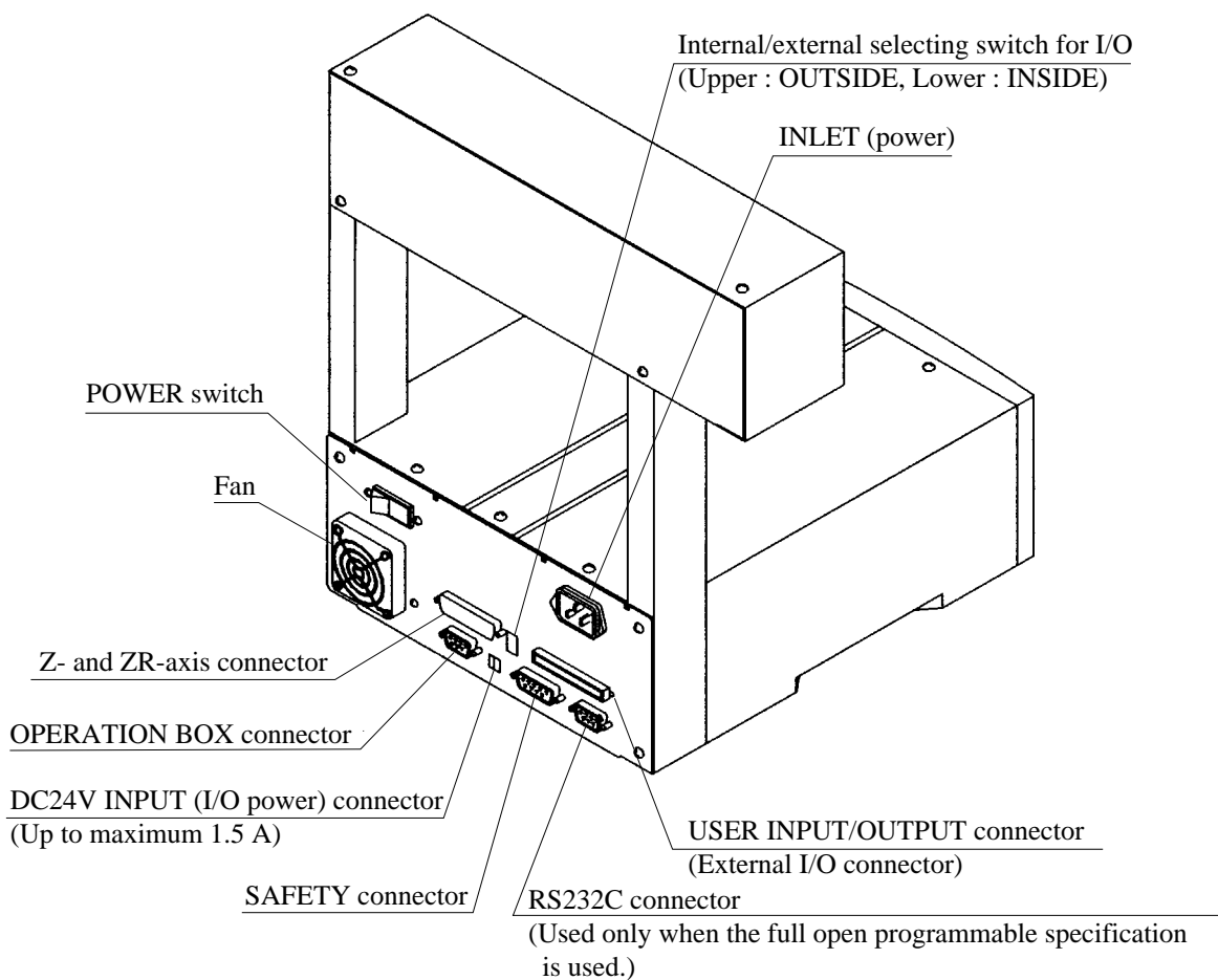
CAST-PRO Teaching Pendant
